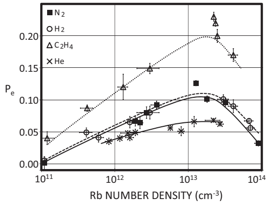
FIG. 3. Source performance with different buffer gases at 200 mTorr in the optical-pumping cell. The values of E_i are \sim 2 and \sim 4 eV for ethylene (see text). Lines serve to guide the eye.
